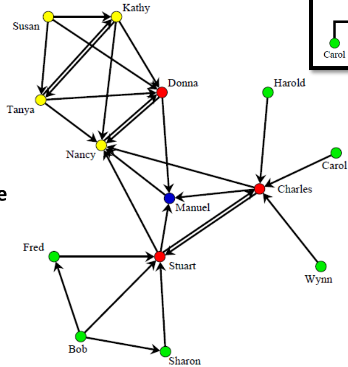
Force-directed layout
